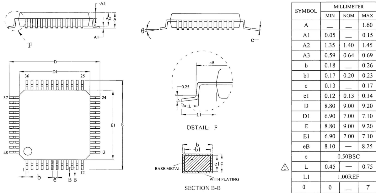
Figure 4-1 JL7031C Package
